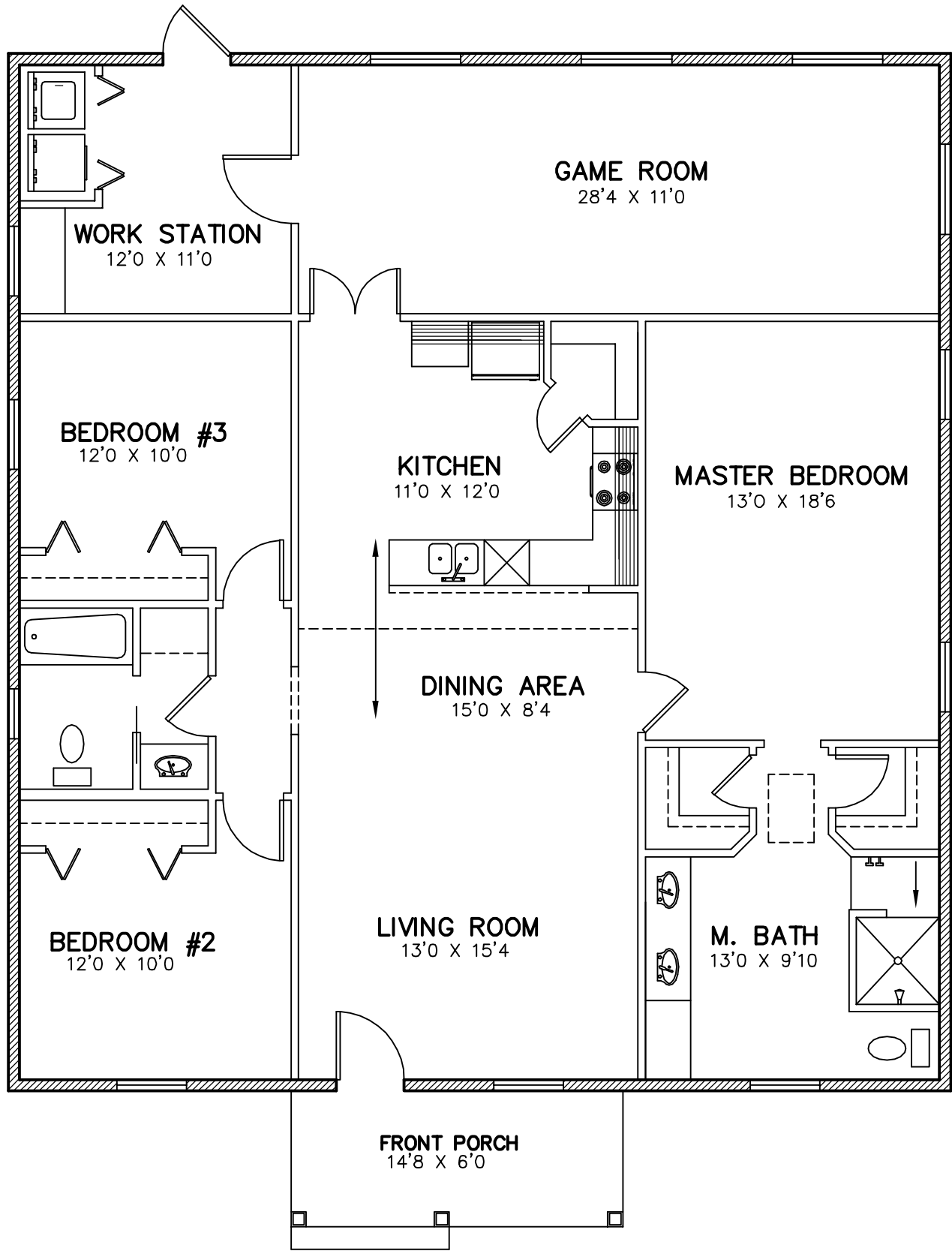
FLOOR PLAN
